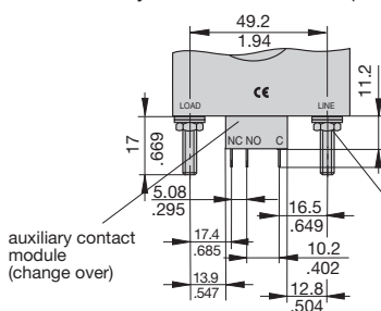
tightening torque: 10-32 UNF, M5 max. 2 Nm 1/4-20 UNC, M6 max. 3 Nm
