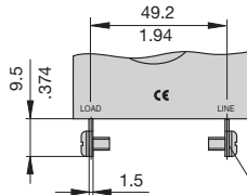
terminal with flat head screw M5 tightening torque max. 1.2 Nm
